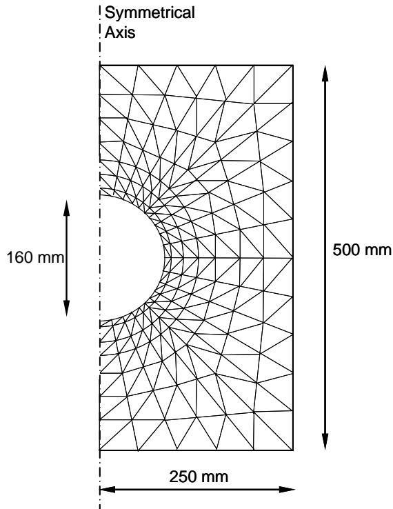
Fig. 2 Finite element mesh
