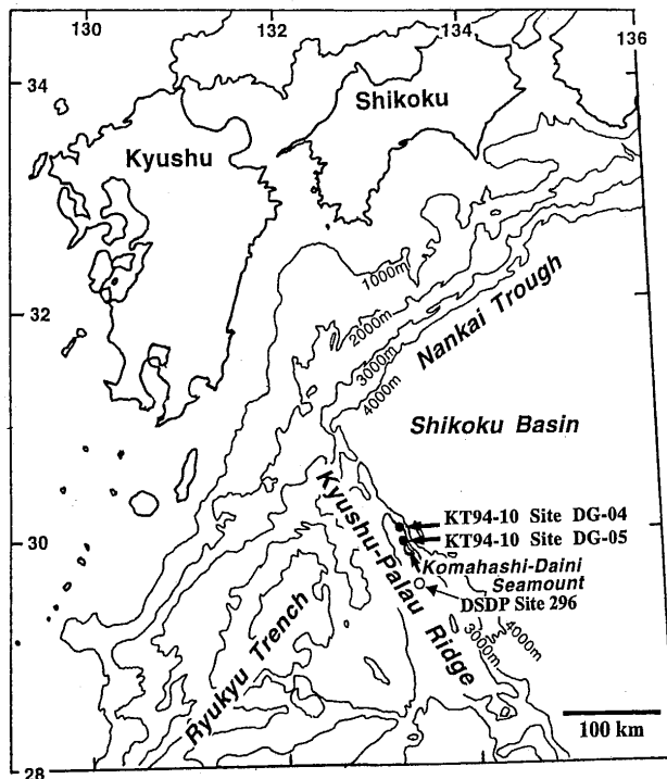
Figure 1. Index map of dredged samples used for this study.
