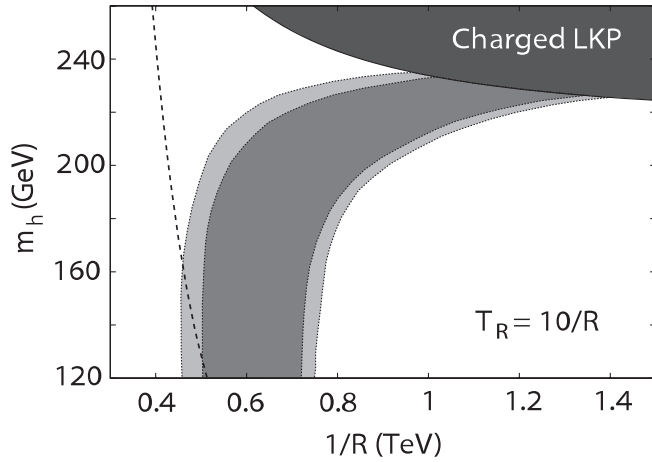
FIG. 3. The parameter region of the model consistent with the WMAP observation in the (1/R, m_h) -plane. The neutrino mass and the reheating temperature are taken as m_\nu = 0-0.66 eV and T_R = 10/R . The dark (light) gray region shows the 1\sigma ( 2\sigma ) allowed region. The dashed line shows the constraint from the electroweak precision measurements [13]. The right side of dashed line is the allowed region (99% confidence level).
