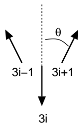
Figure 5. Classical noncollinear spin configuration.
