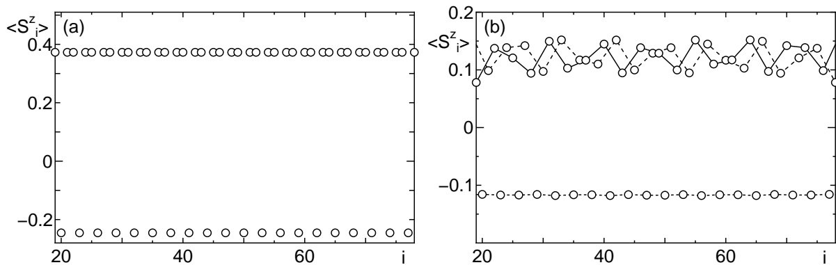
Figure 4. Local magnetization profile (a) in the Lieb-Mattis type ferrimagnetic phase with \delta = 0.7 and \alpha = -0.7 and (b) in the noncollinear ferrimagnetic phase with \delta = 0.8 and \alpha = -0.39 for N = 96 calculated by DMRG method. Only the sites in the middle of the system 19 \leq i \leq 78 is shown to exclude the boundary effects. The lines are guides for eye drawn to make clear the incommensurate modulation of the magnetization profile.
