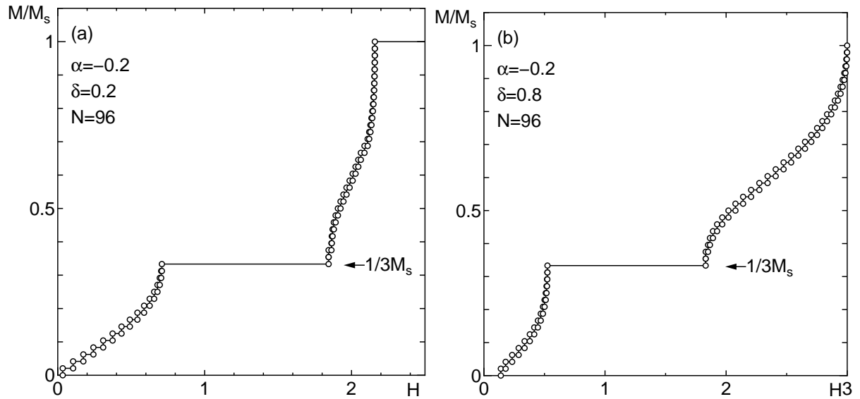
Figure 2. Magnetization curve in (a) Tomonaga-Luttinger liquid phase with (\delta, \alpha) = (0.2, -0.2) and (b) Majumdar-Ghosh type dimer phase with (\delta, \alpha) = (0.8, -0.2) for N = 96 calculated by DMRG method.
