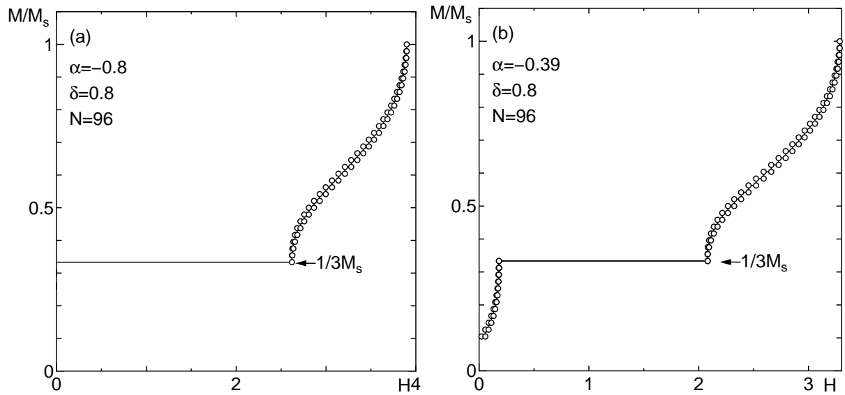
Figure 3. Magnetization curves in (a) Lieb-Mattis type ferrimagnetic phase with (\delta, \alpha) = (0.8, -0.8) and (b) noncollinear ferrimagnetic phase with (\delta, \alpha) = (0.8, -0.39) for N = 96 calculated by DMRG method.
