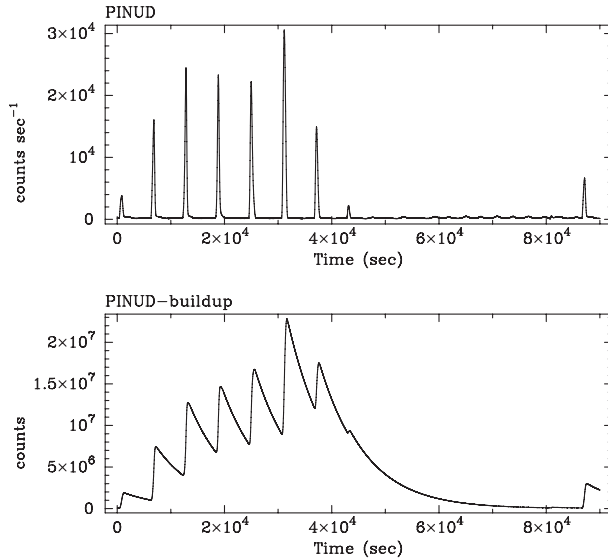
Fig. 4. Example of PINUD-buildup. The top panel shows the light curve of the PINUD count rate in units of counts s -1 per one unit (4 PINs), and the bottom shows the PINUD buildup convolved with a time constant of 8000 s.
