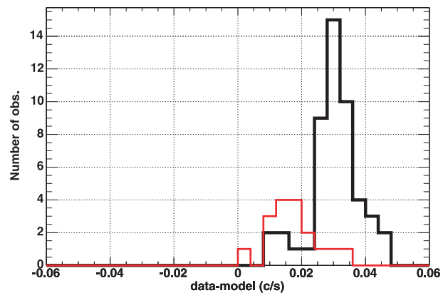
Fig. 13. Same as figure 12, but observations of E0102 (black) and Cygnus Loop multi-pointing (red) are used and results for the background model LCFITDT are shown.
