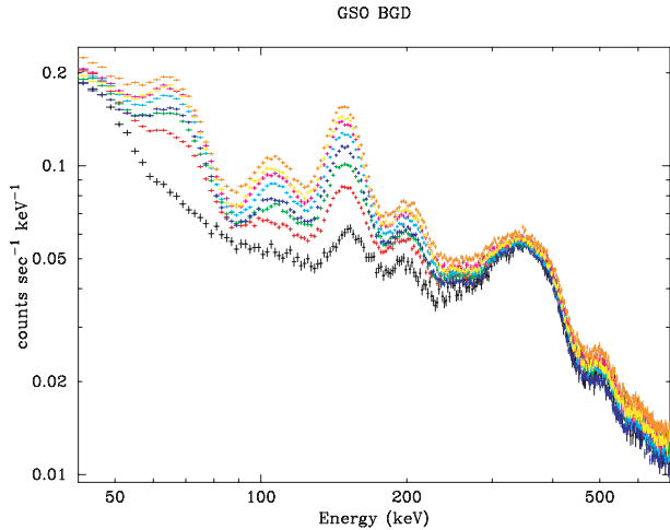
Fig. 3. Comparison of the GSO NXB spectra using Earth occultation data in different epochs; 2005-08-31, 2005-12-03, 2006-03-09, 2006-06-13, 2006-09-26, 2007-01-05, 2007-04-10, and 2007-08-09 from bottom to top.
