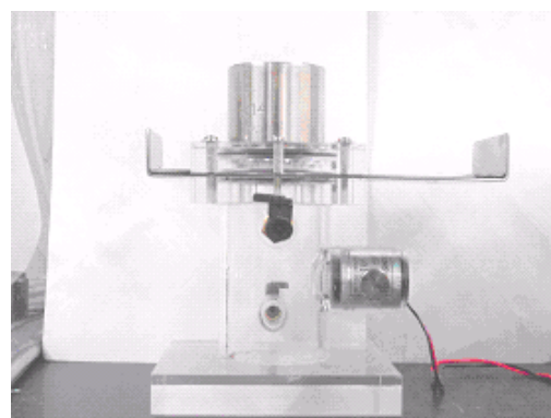
Fig. 3 Gas diffusivity measurement device.
