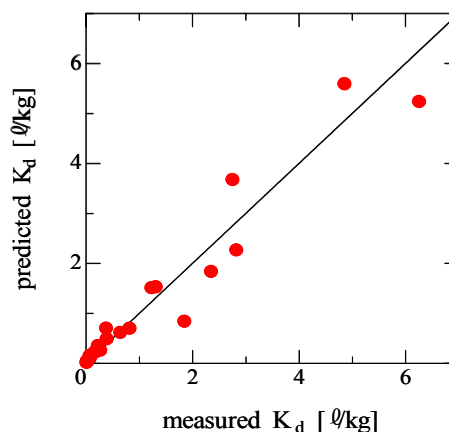
Fig. 4 Comparison between measured absorption coefficients ( K_d ) for 2,4-D and predicted values by the proposed predictive model.
